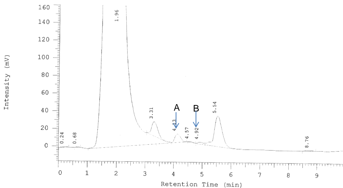
Figure 4 HPLC chromatogram of H. hemerocallidea . R T A- 4.13 (ergosterol), R T B- 4.92 (stigmasterol),
