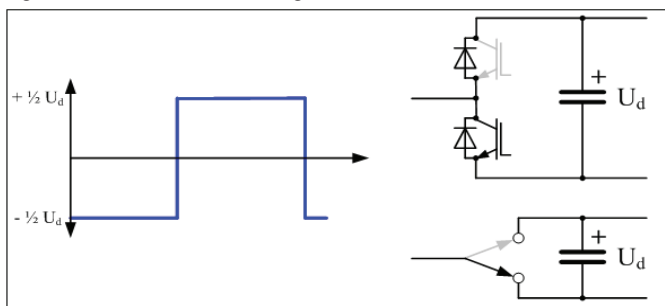
Fig. 2. Block diagram of a two-level VSC-HVDC
