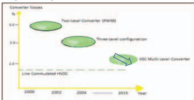
Fig. 11. LCC and VSC power loss
