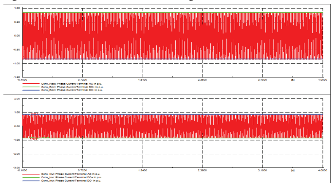
Fig. 10. VSC-Converter current
