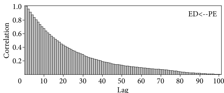
Fig. 6. Posterior correlation plot of the MGNREGP QUAL Regression Model for the Mediated Factor Economic Development and Poverty Eradication Source: Authors' own creation.
