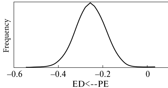
Fig. 4. Posterior frequency polygon distribution of the Mediating Factor Economic Development and Poverty Eradication Source: Authors' own creation.
