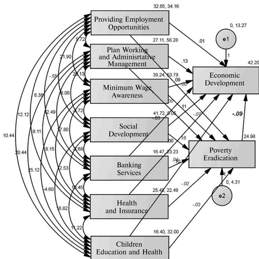
Fig. 3. Shows The AMOS Output with Regression Weights of “MGNREGP QUAL” Mediated Model
