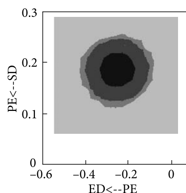
Fig. 7. Two-dimensional plot of the bivariate posterior density for the Regression Weights Social Development to Poverty Eradication and Economic Development Source: Authors' own creation.
