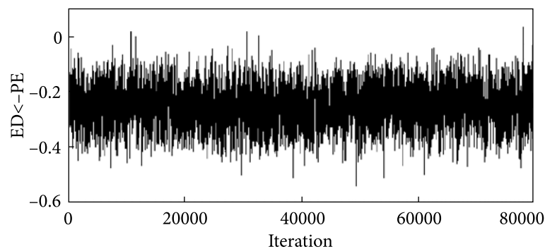
Fig. 5. Posterior trace plot of the MGNREGP QUAL Regression Model for the Mediated Factor Economic Development and Poverty Eradication Source: Authors' own creation.
